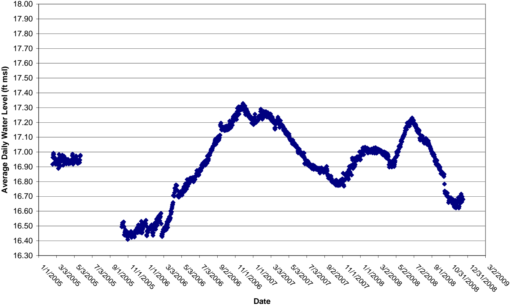
Kunia Mauka Deep Monitor Well, Oahu (2503-01) - Average Daily Water Levels
