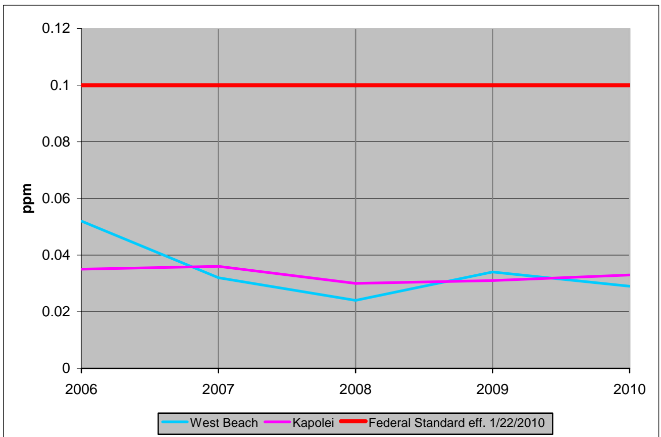
Figure 7-8. NO 2 Maximum 1-Hour Average: 2006 – 2010
