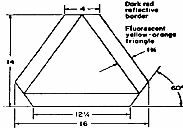
FIGURE J-7.—SLOW-MOVING VEHICLE EMBLEM
