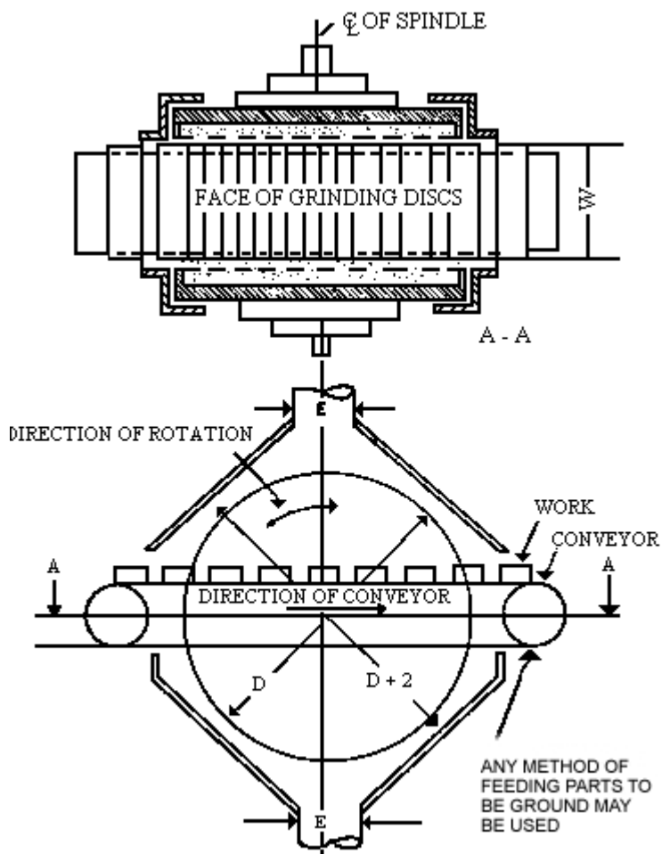
FIGURE G-7 HORIZONTAL DOUBLE-SPINDLE DISC GRINDER EXHAUST HOOD AND BRANCH PIPE CONNECTIONS
