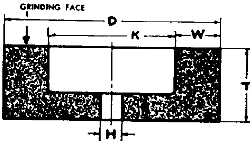
Type 6—Straight-cup Wheel
