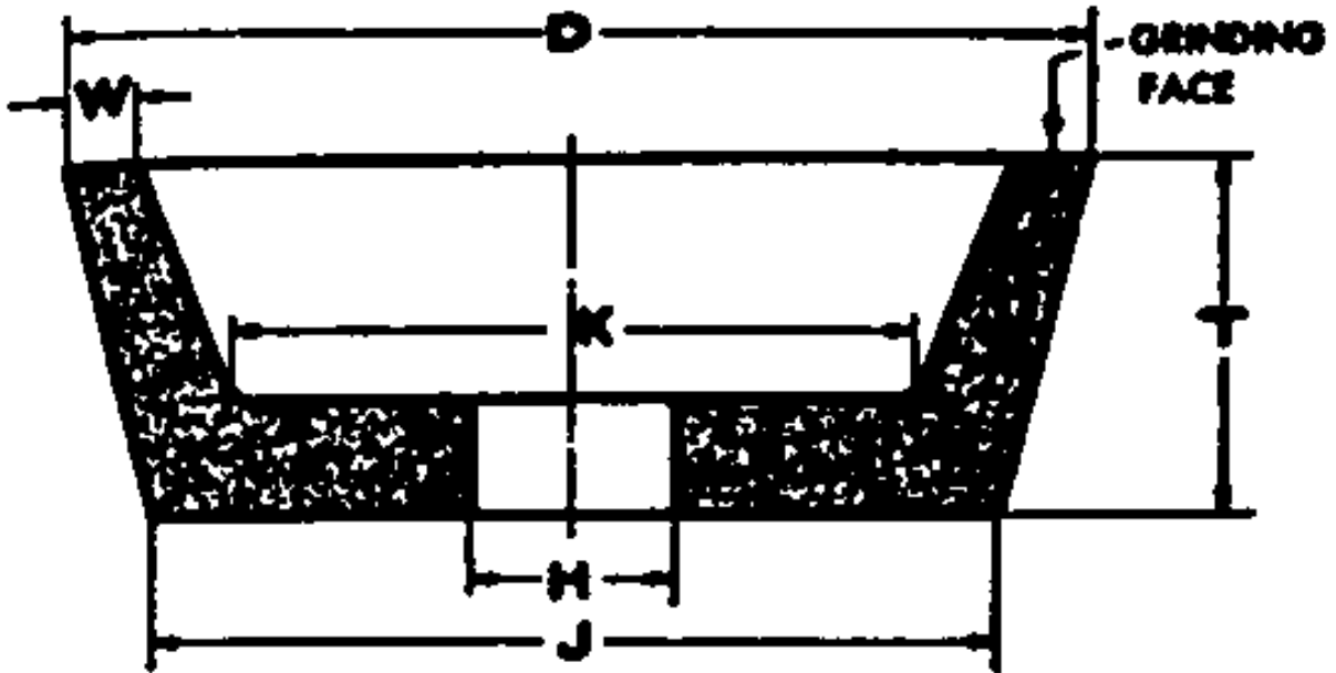
Type 11—Flaring-cup Wheel
